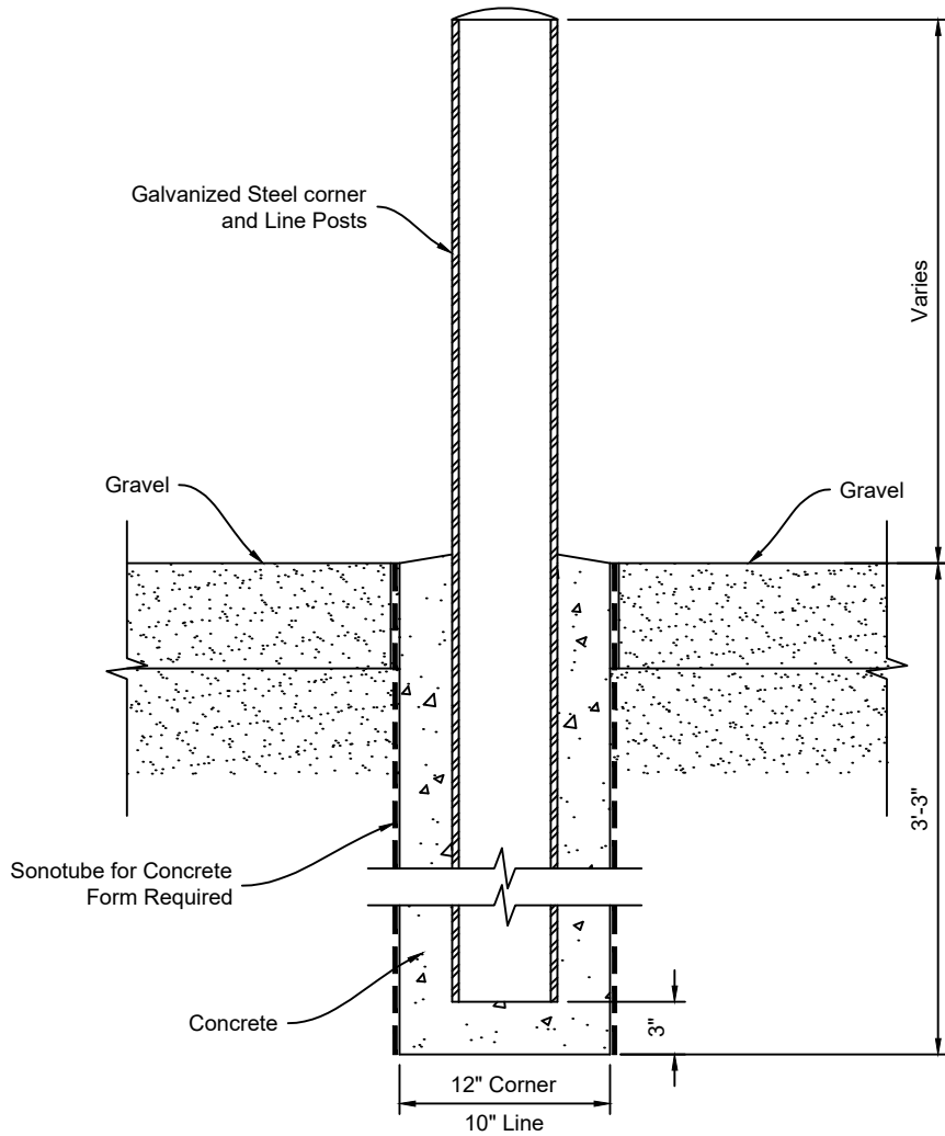
CHAIN LINK FENCE POST FOOTING DETAIL
